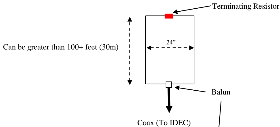
Fig 2.1.1 Single loop
